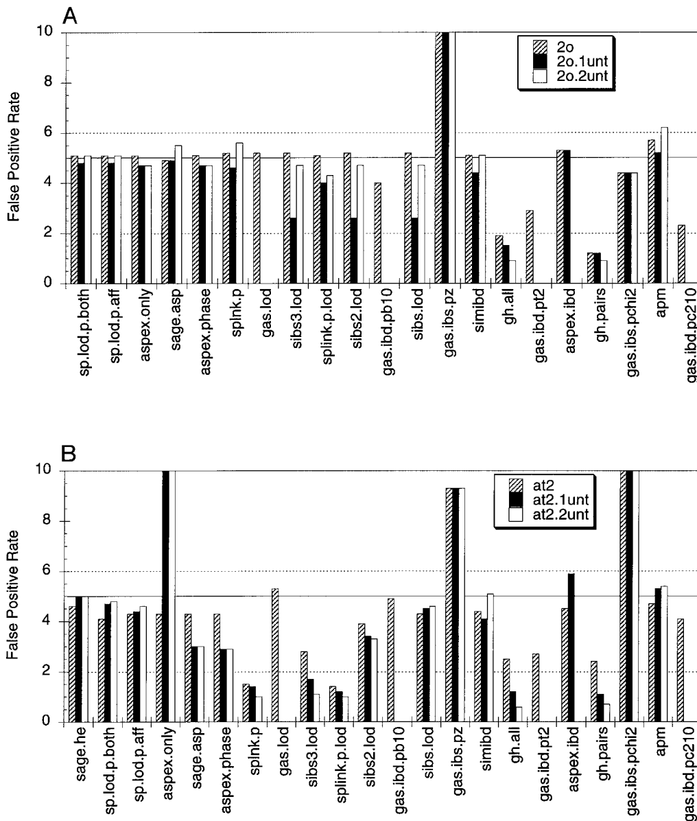
Figure 2 False-positive rates. Statistics are ordered in decreasing rank, by power, with the best-ranked statistic on the left (as in fig. 1). For definitions of the statistic names, see table 1. A, Family structure included two affected siblings and their parents, with zero (“2o”), one (“2o.1unt”), or both (“2o.2unt”) parents untyped. B, Family structure included four siblings, at least two of whom were affected, and their parents, with zero (“at2”), one (“at2.1unt”), or both (“at2.2unt”) parents untyped.
